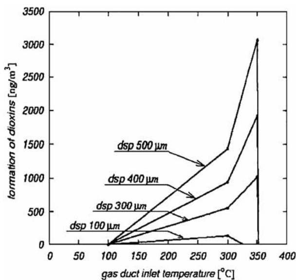
Fig. 2. Alterations of dioxin formation depending on spray water droplet and inlet gas temperature.
