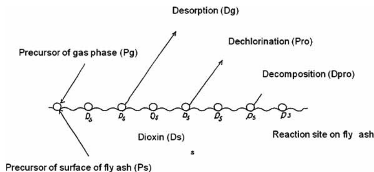
Fig. 1. Scheme of dioxin formation and its degradation pathway.
